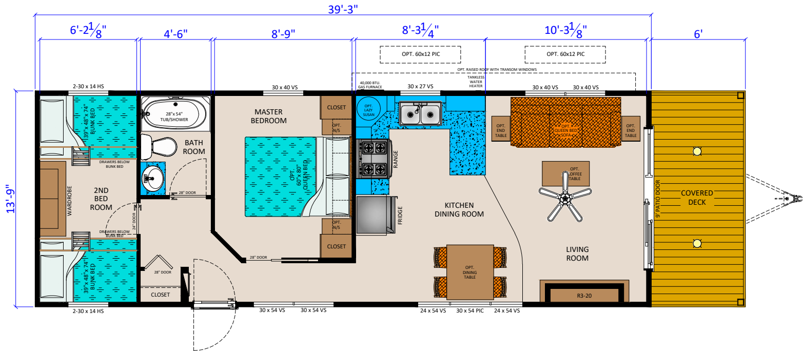
ROSEDALE 20 (R3914 2BR FL) (540 SQ.FT.)
